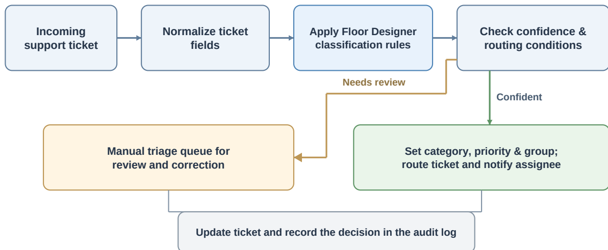
Figure 1: Designer-based workflow for classifying and routing incoming support tickets
